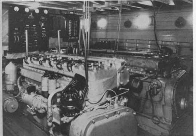
Lady Isabel a 68-footer owned by Mr. L. E. Muttart. This yacht was designed and built by New York Yacht, Launch & Engine Co. and has twin Sterling Petrels
